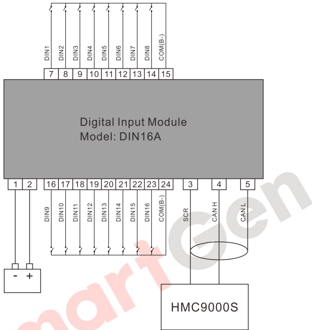
Fig.2 Typical Wiring Diagram
