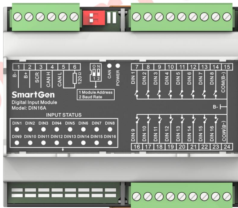
Fig.1 DIN16A Panel
