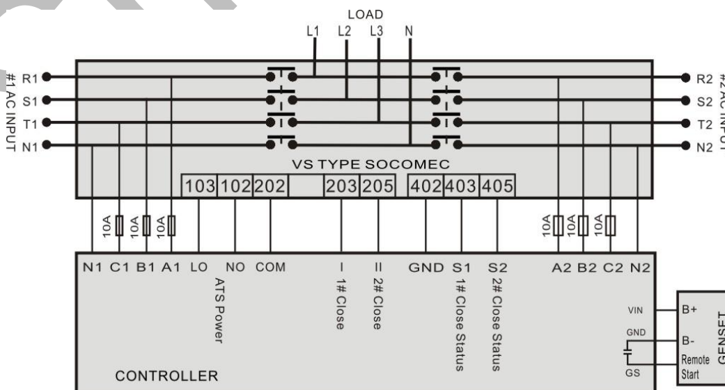
SOCOMECS VS Type Switch
