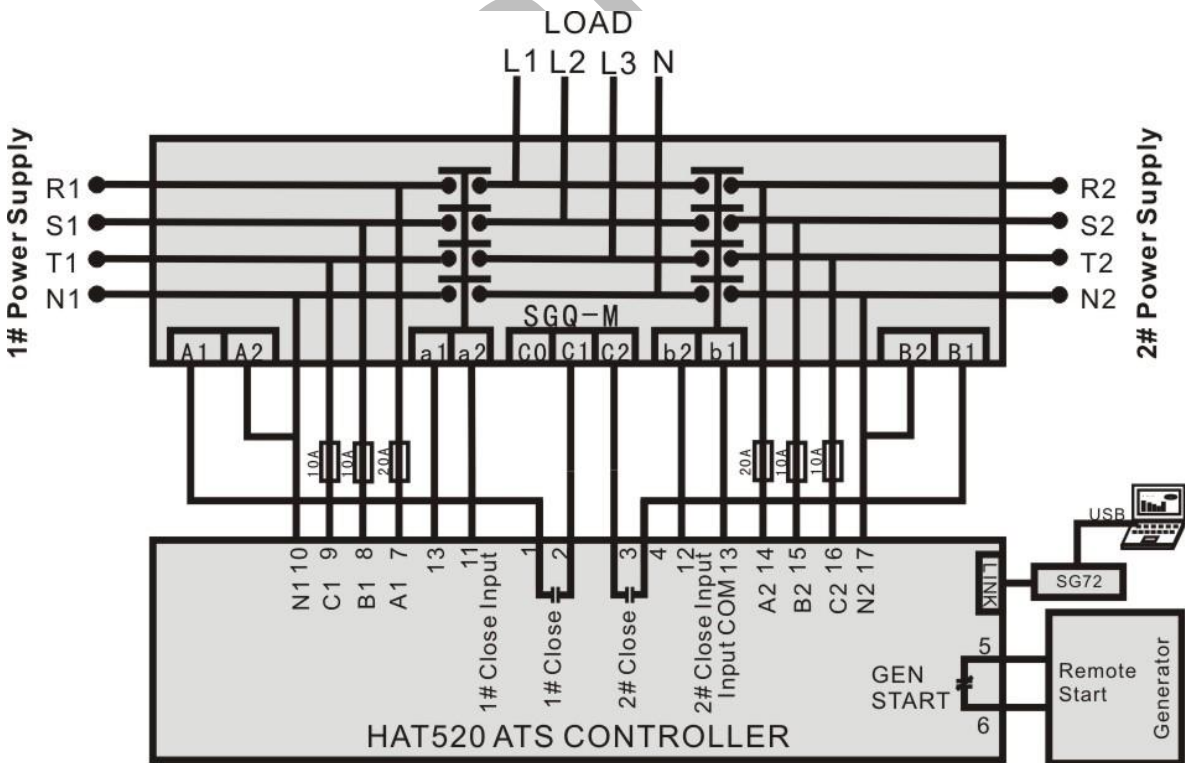
SGQ-M Wiring Diagram
