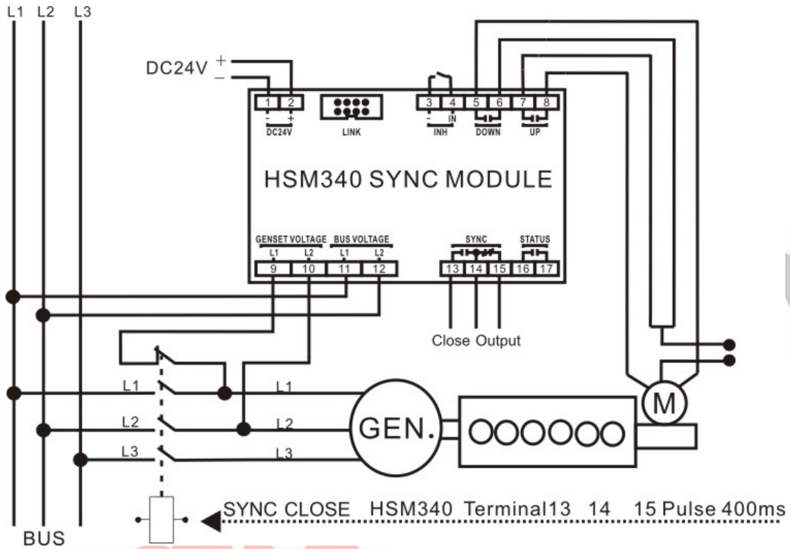
Fig. 4 - HSM340 3Phase 3Wire Typical Application
