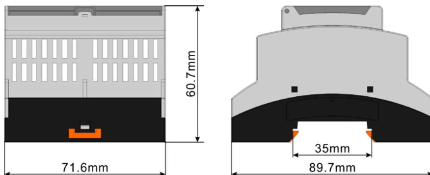
Fig.5 - Overall Dimensions
