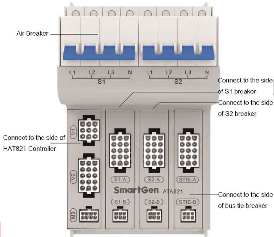
Fig. 1 Panel Instruction
