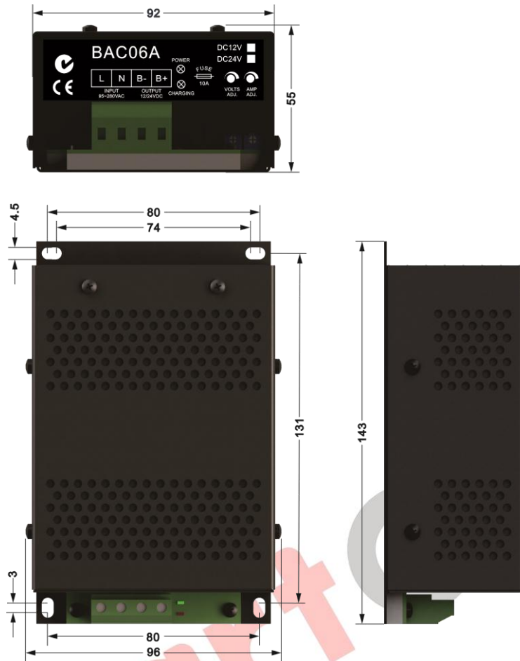
Chart 3. BAC06A Dimension
