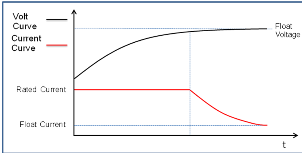
Fig. 1 Charging Principle
