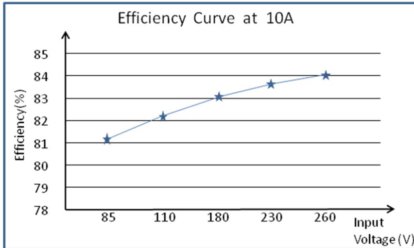
Fig. 2 Efficiency Curve
