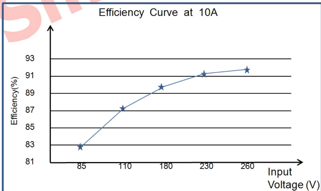
Fig.2- Efficiency Curve
