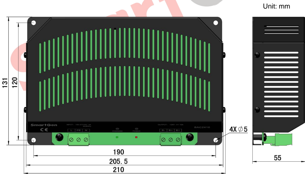
Fig.4- BAC2410 Case Dimensions
