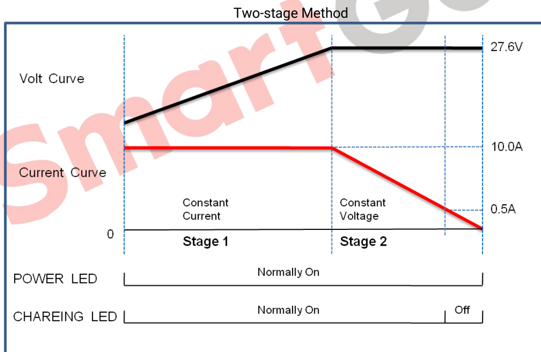
Fig.1- Two-stage Charging Method
