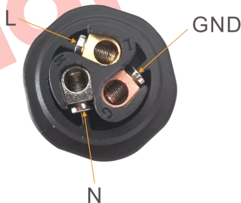
Fig. 5 Wire Connection
