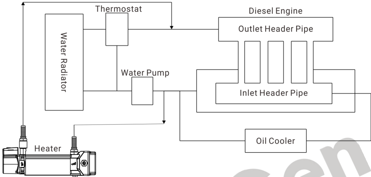
Fig. 1 - Installation Logic Diagram
