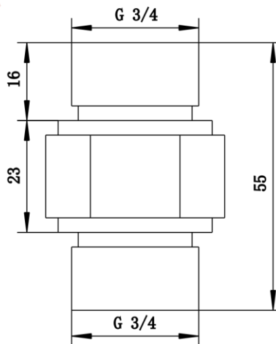
Fig. 9 Pair Screw Size
