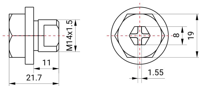
Fig. 6 Vent Valve Size
