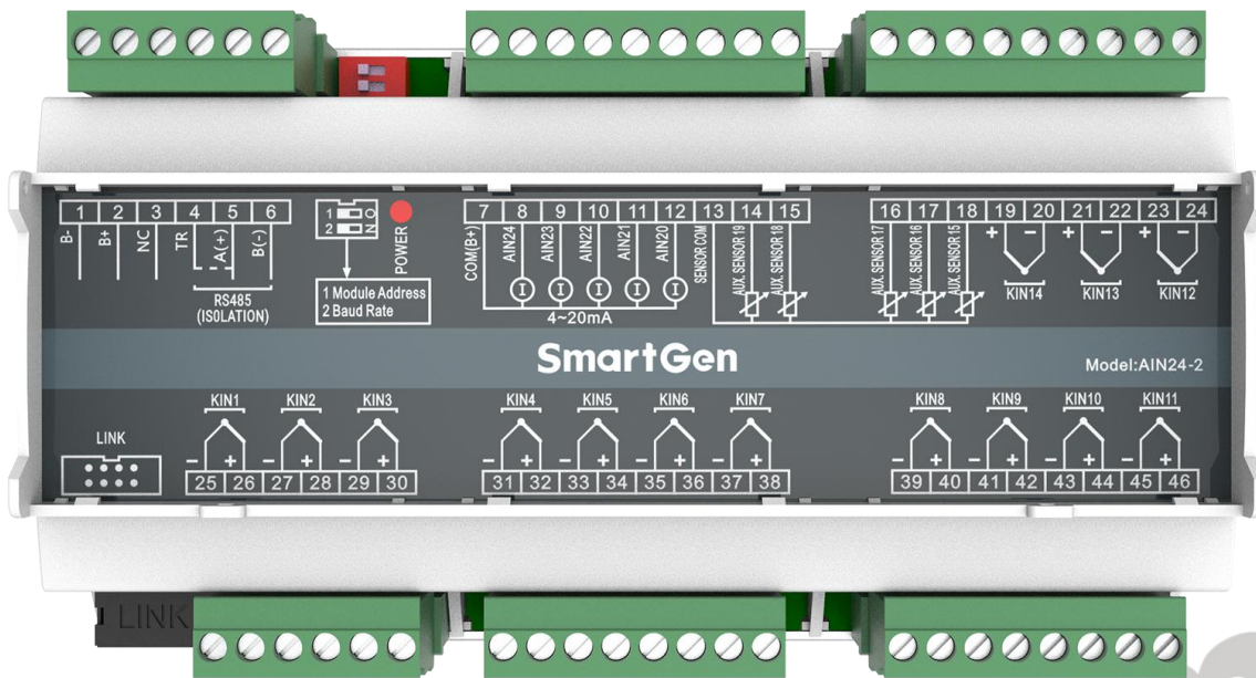
Fig. 1 – AIN24-2 Panel Drawing
