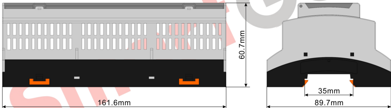
Fig.3 – Overall Dimensions
