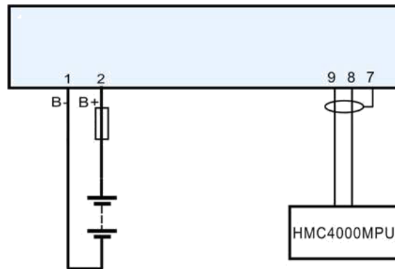
HMC4000RM Typical Application
